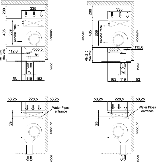
Standard Installation
